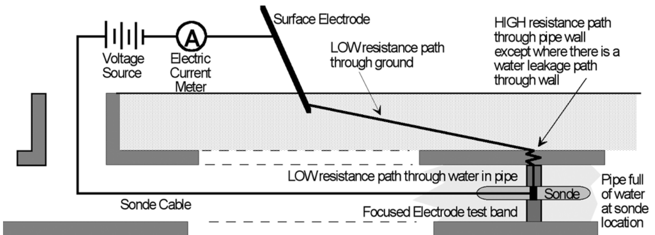
FIG. 1 Electro-scan Electrical Schematic
