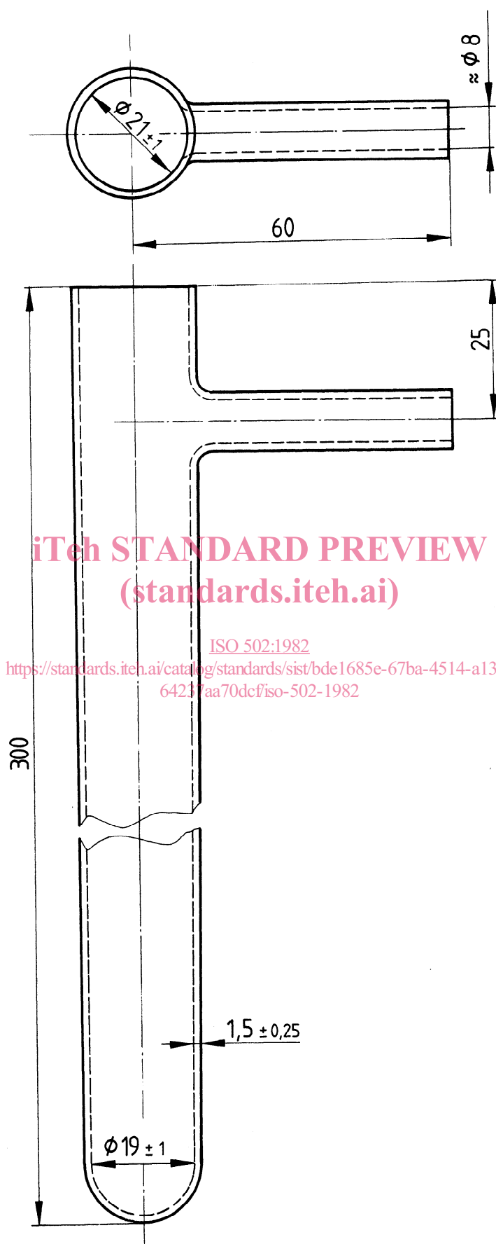
Figure 4 – Retort tube
