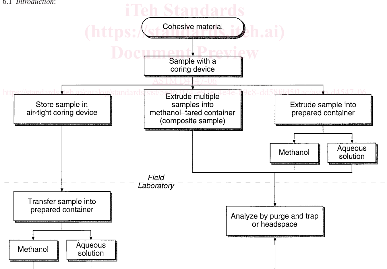
FIG. 1 Sample Handling Options for Cohesive Materials
