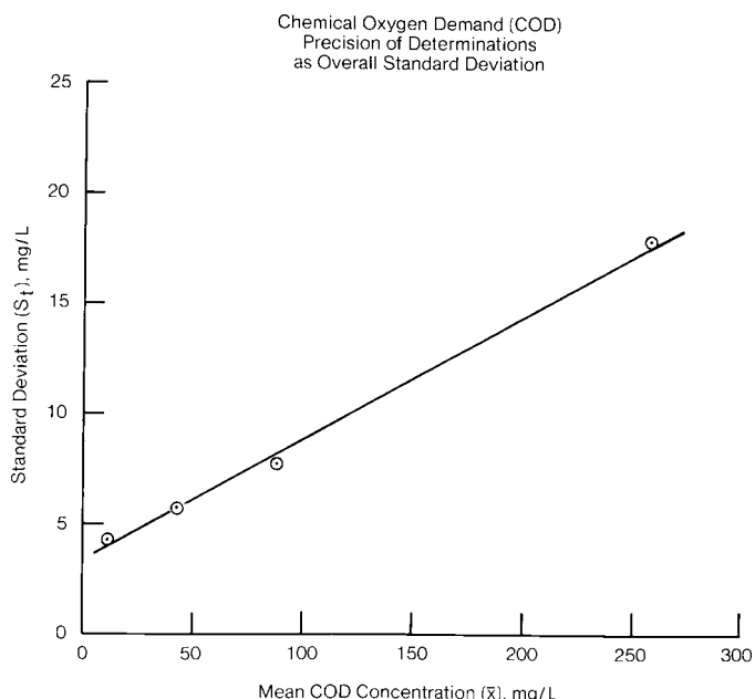
FIG. 1 Test Method A, Chemical Oxygen Demand (COD) Precision of Determination as Overall Standard Deviation
