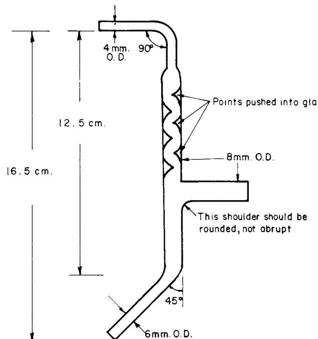
FIG. 3 Microdistillation Column
