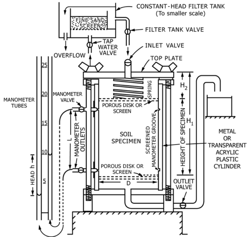
FIG. 1 Constant-Head Permeameter
