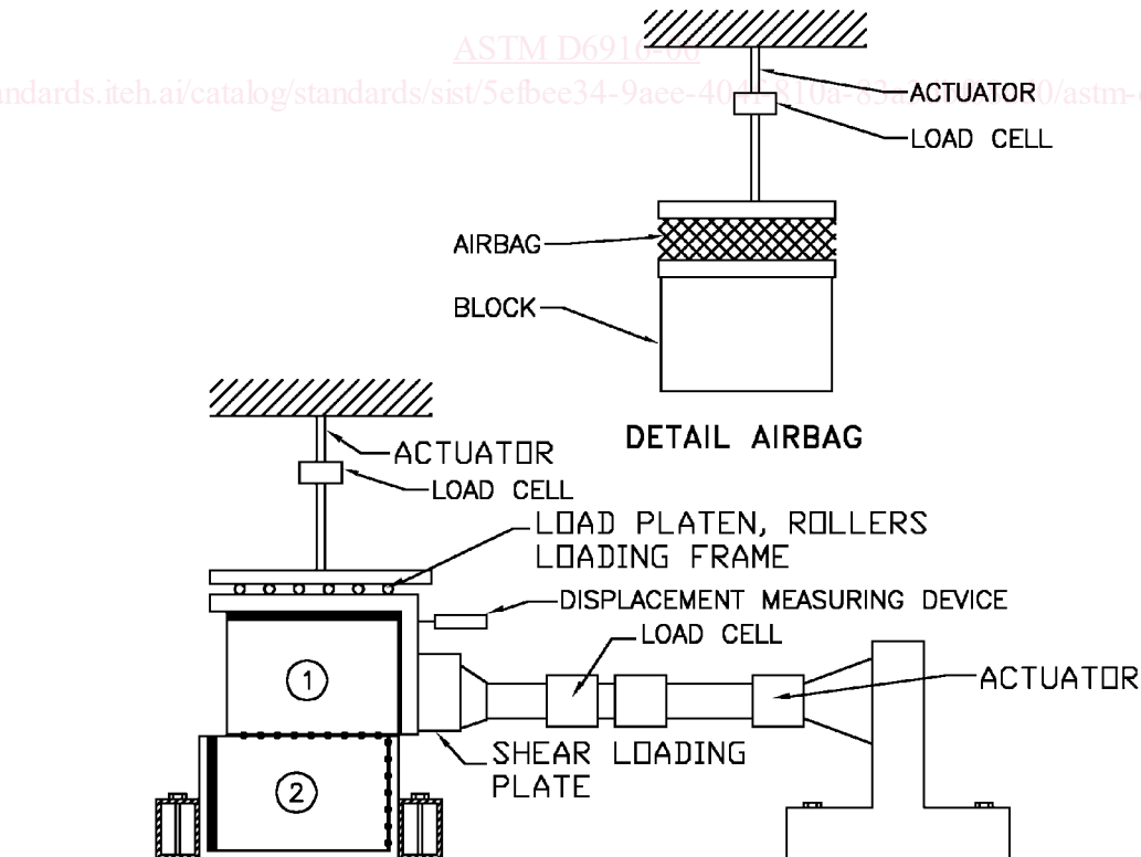
FIG. 1 Connection Test Apparatus (Plan View)
