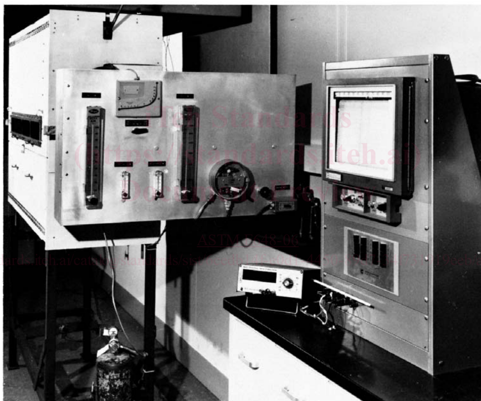
FIG. 1 Flooring Radiant Panel Tester Apparatus
