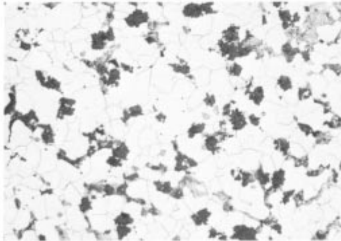
FIG. 1 Reference Photomicrograph Showing Allowable Pearlite in Grade M3210 Iron (100 ×; 2 percent Nital Etch)
