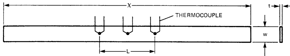
FIG. 4 Example of Emittance Sample in the Test Fixture
