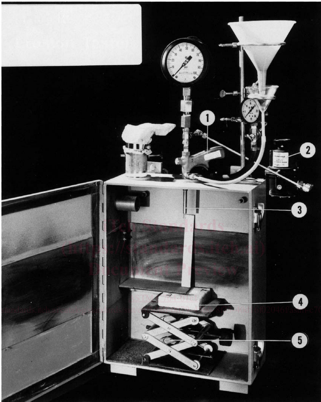
FIG. 2 Abrasion Tester
