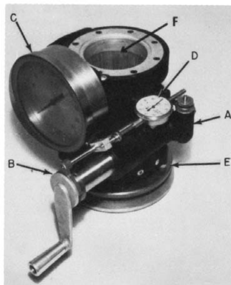
A—Air cell. B—Displacement pump. C—200-psi pressure gage. D—Ames dial. E—Base adjustment nut. F—Bottom of upper tapered ring.
