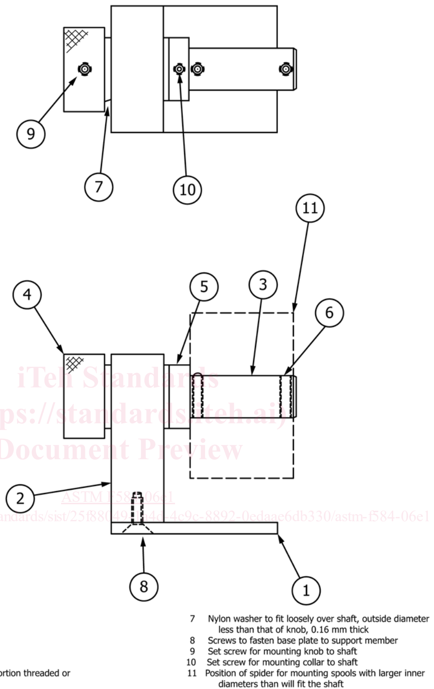
FIG. 2 One Form of Spool Inspection Jig
