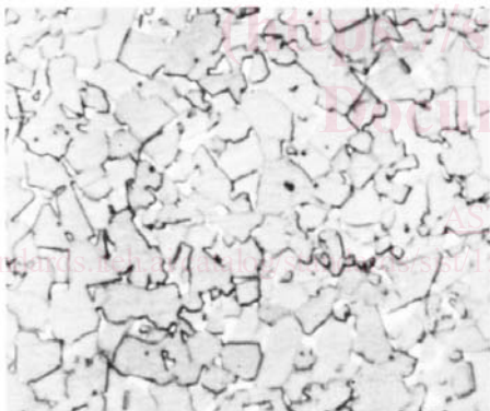
FIG. 1 Apparent Grain Size of Tungsten Carbide plus 6 % Cobalt (1500×)
