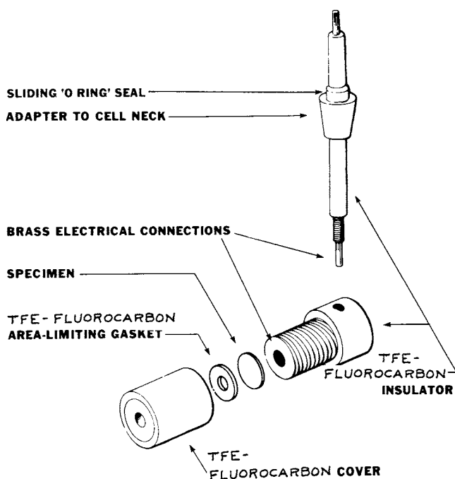
FIG. 1 Schematic Diagram of Specimen Holder 1,1
