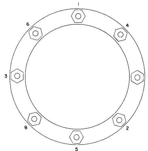
NOTE—Tighten bolts evenly; follow numerical sequence. FIG. 2 Bolt Tightening Progression
