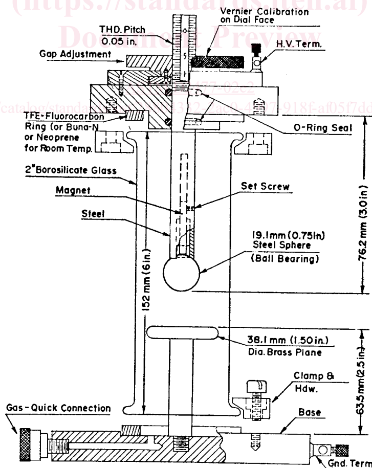
FIG. 1 Test Cell
