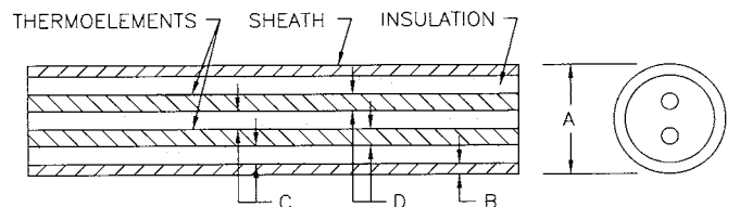
FIG. 7 Sheathed Thermocouple Construction
