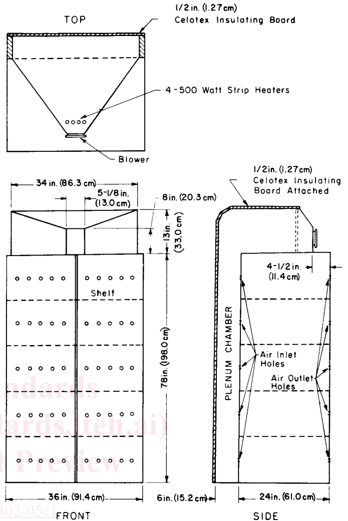
FIG. 2 Air-Drying Oven
