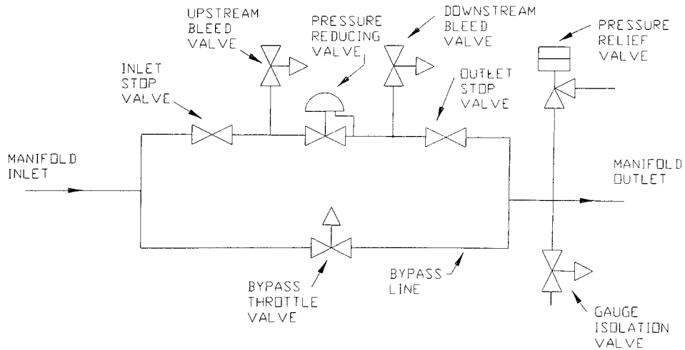
FIG. 1 Manifold Configuration
