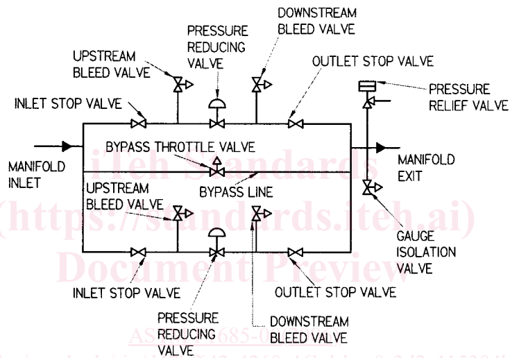
FIG. 2 Manifold Configuration
