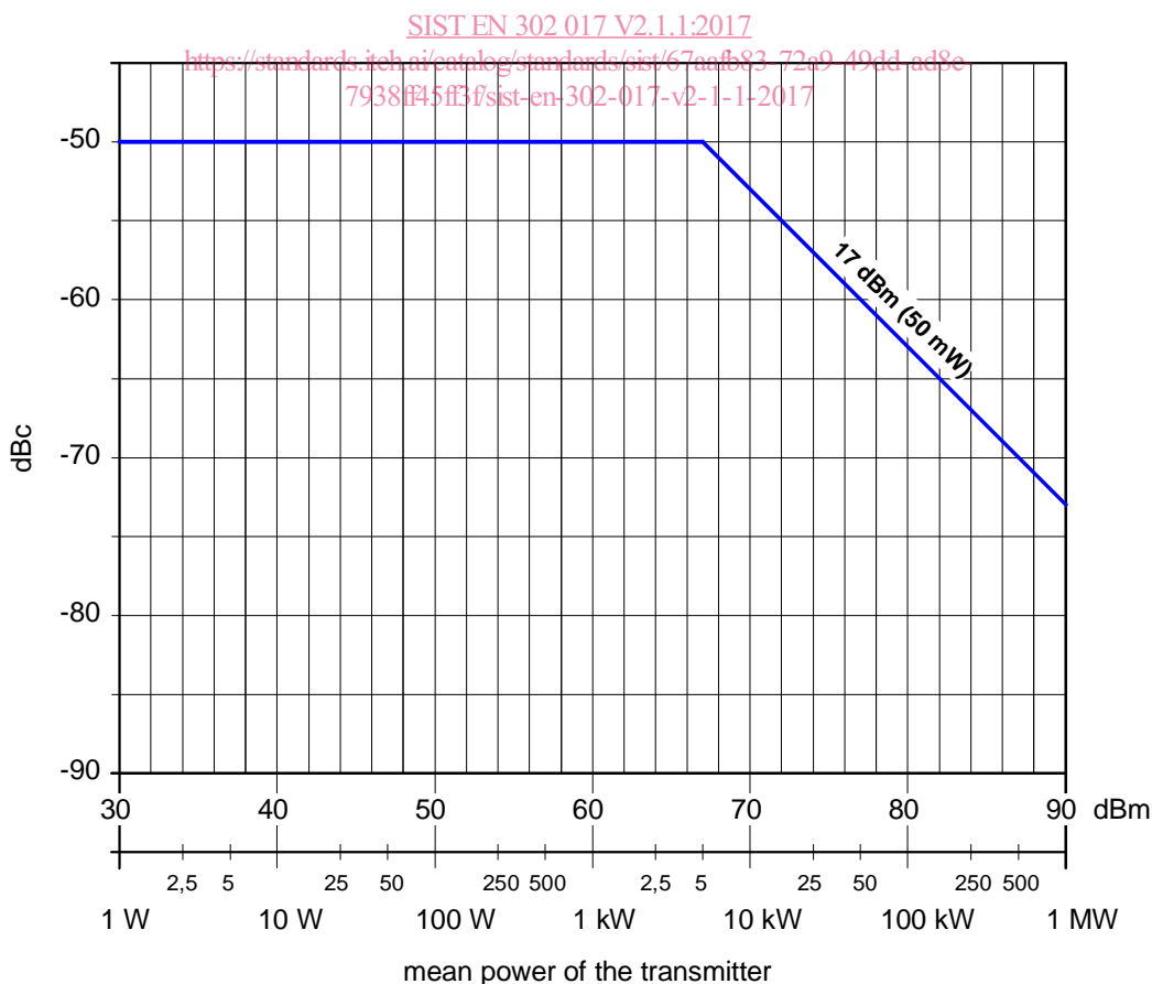
Figure 4.1: Spurious emission limits
