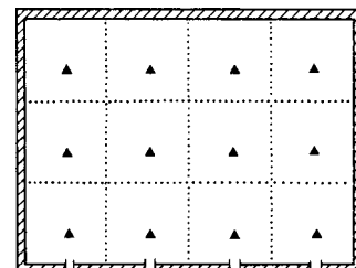
FIG. 1 Traverse Positions for Rectangular Flue
