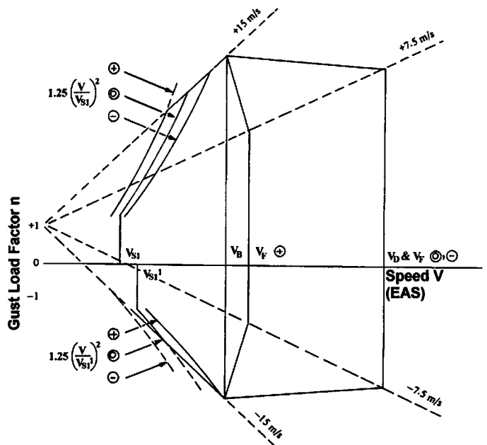
FIG. 2 Gust Envelope
