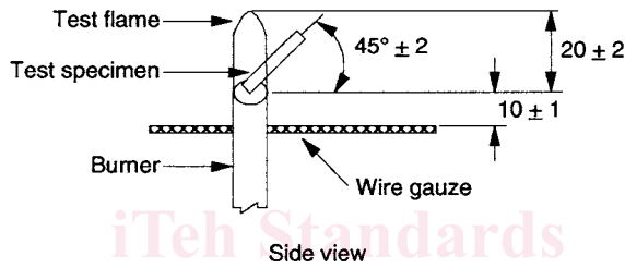
FIG. 1 Test Fixture
