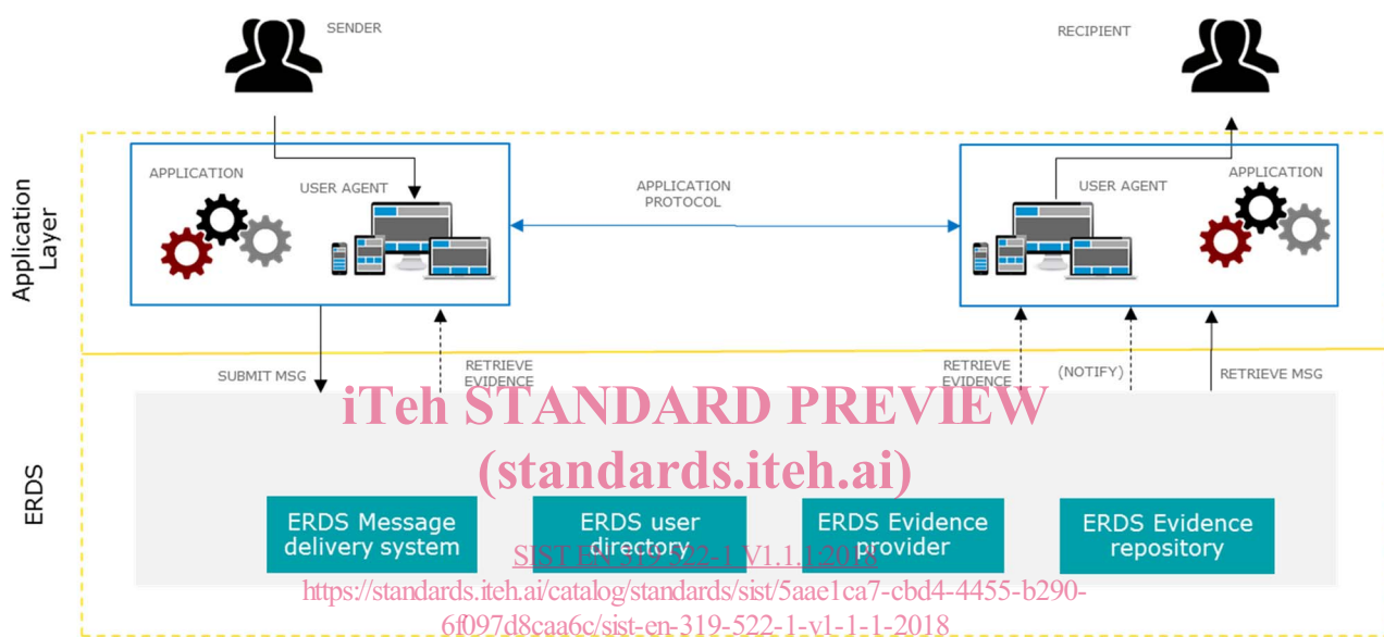
Figure 1: Black-box registered delivery service model
