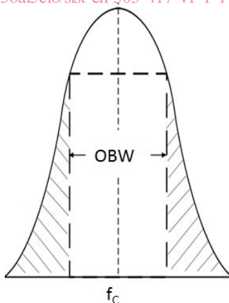
Figure 1: Occupied bandwidth (OBW)
