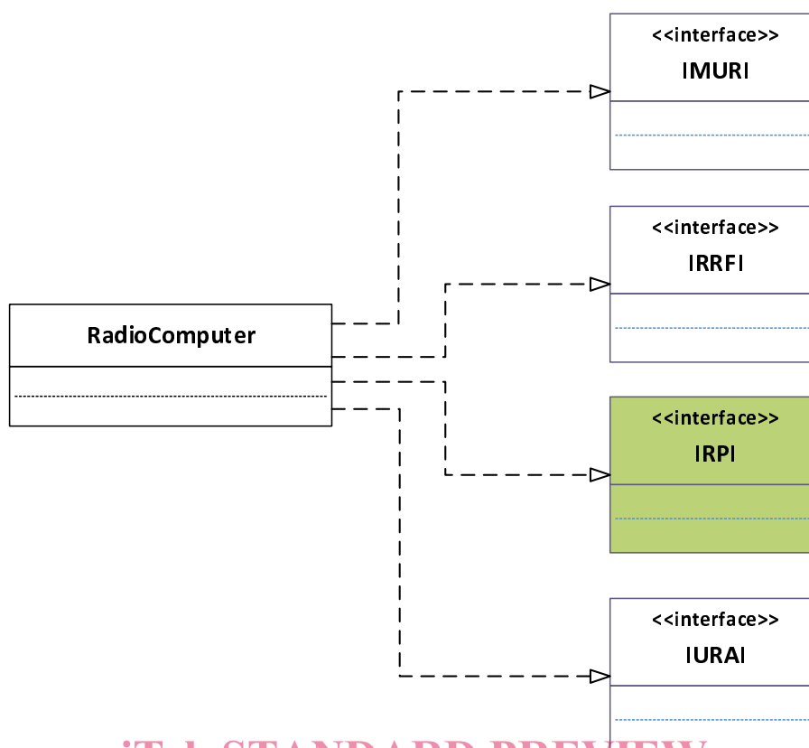
Figure 4.2: UML® class diagram for Radio Computer interfaces (standards.iteh.ai)
