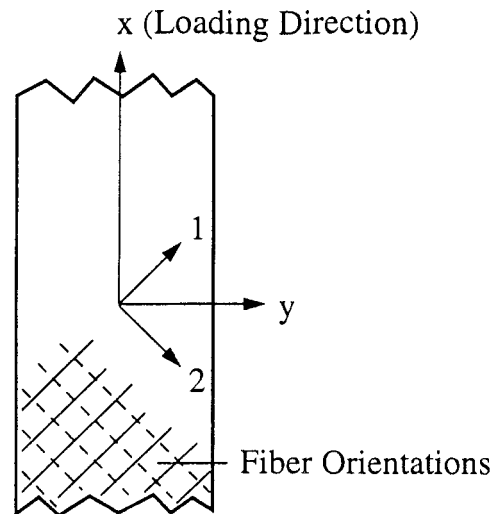
FIG. 2 Definition of Specimen and Material Axes
