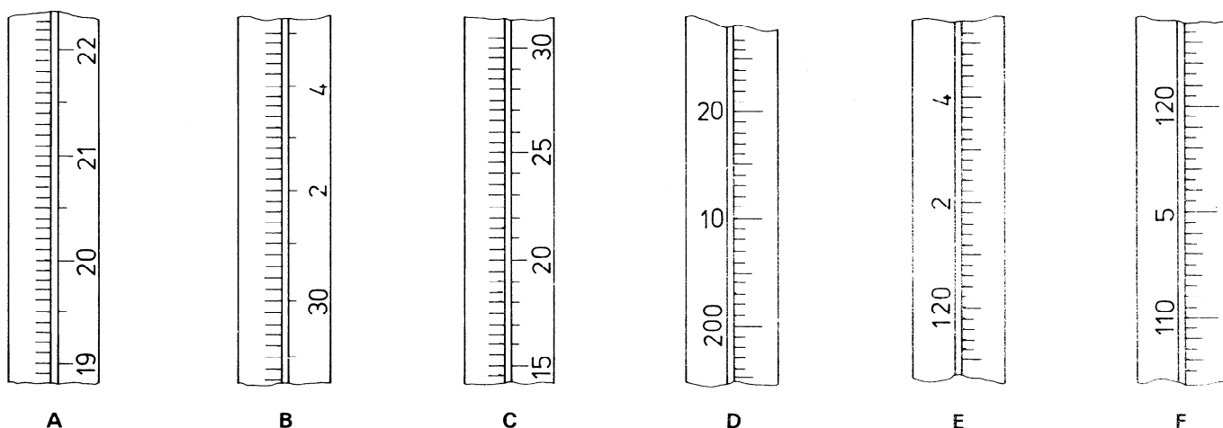
Figure 2 — Alternative types of graduation and figuring
