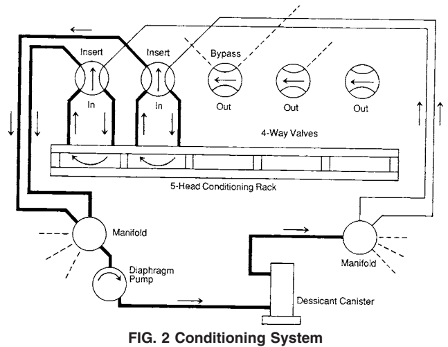
FIG. 2 Conditioning System
