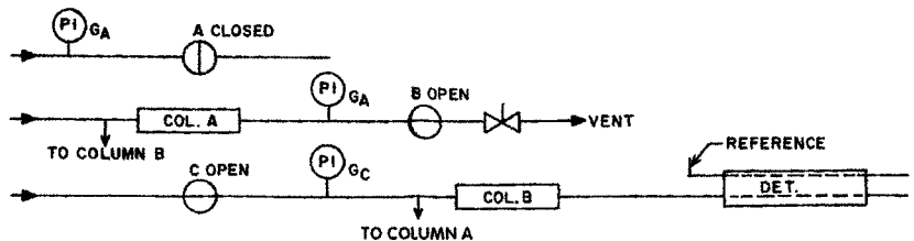
FIG. 1 Pressure Backflush
