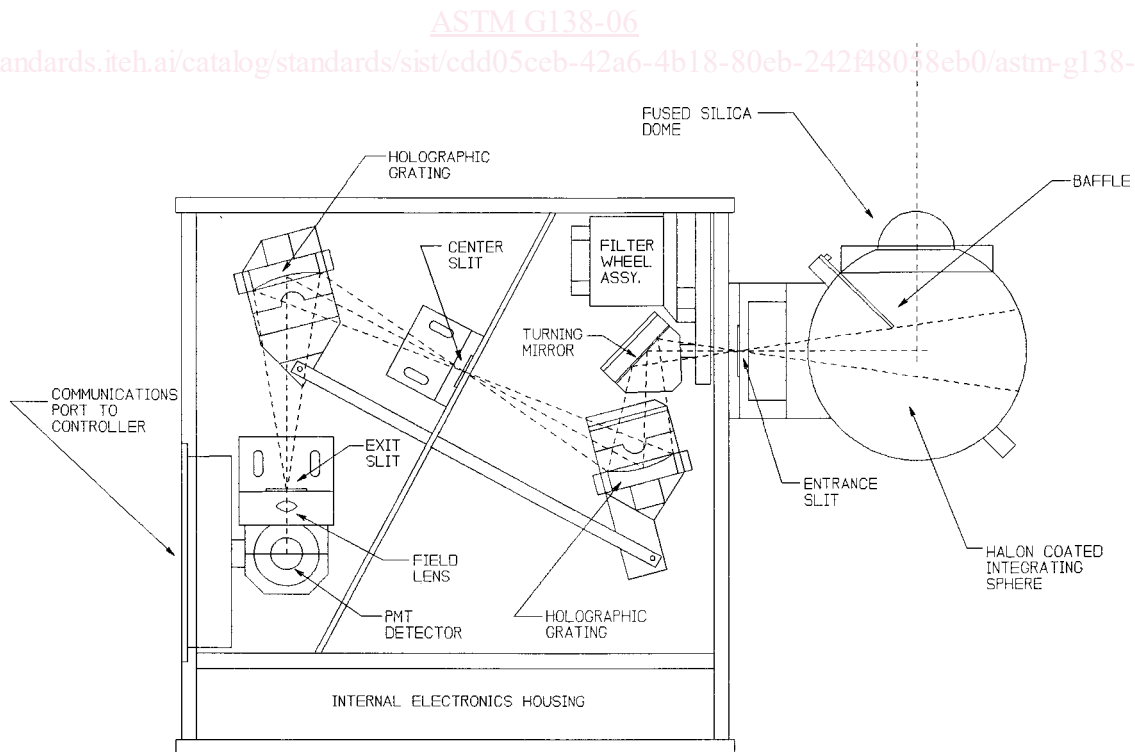
FIG. 1 Typical Double Grating Monochromator Layout
