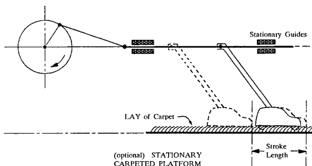
FIG. 1 Test Fixture
