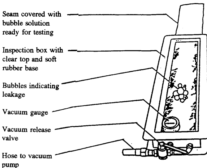
FIG. 1 Vacuum Chamber
