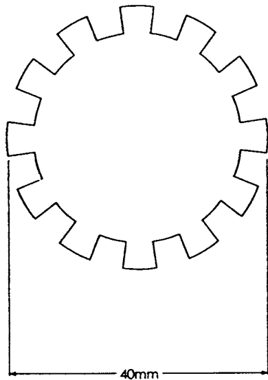
FIG. 2 Distributor Plate
