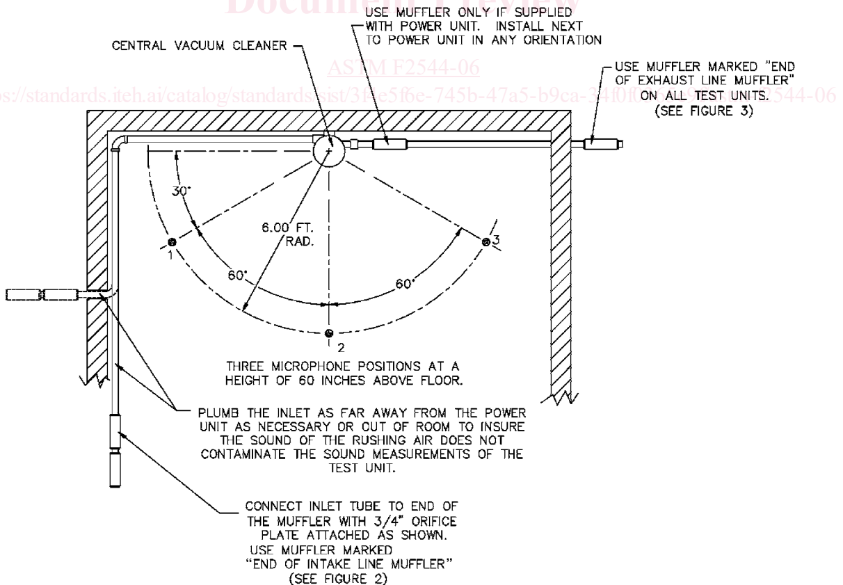
FIG. 1 Sound Test Layout
