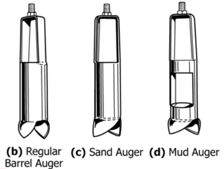
FIG. 5 Barrel Auger Variations and Soil Moisture
