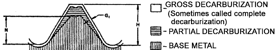
FIG. 1 Decarburization Zones
