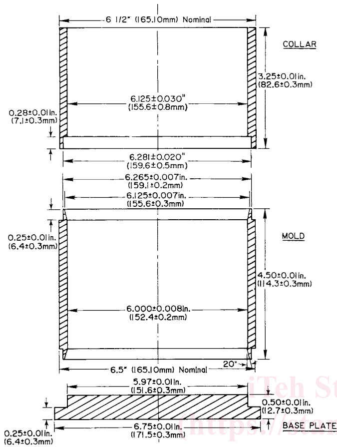
FIG. 1 Compaction Mold
