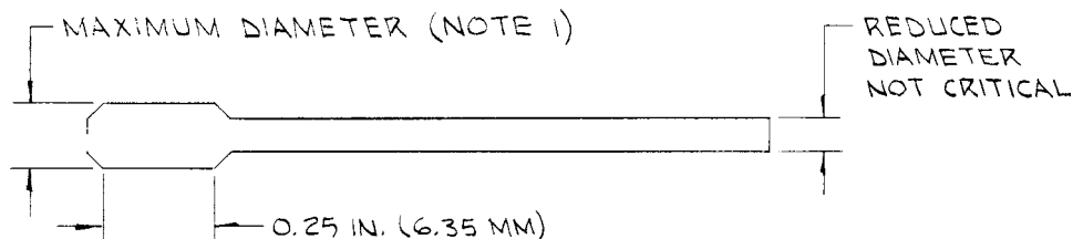
FIG. 1 Barrel Performance Test Gage
