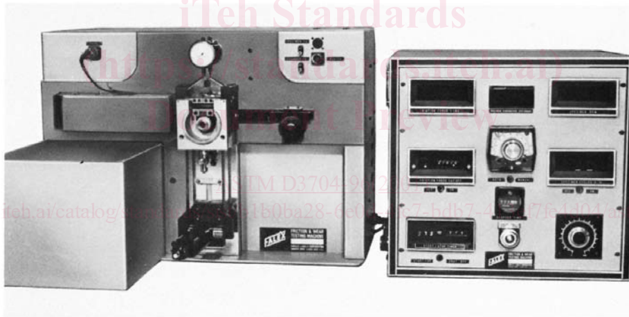
FIG. 1 Failex Ring and Block Test Machine (continued)
