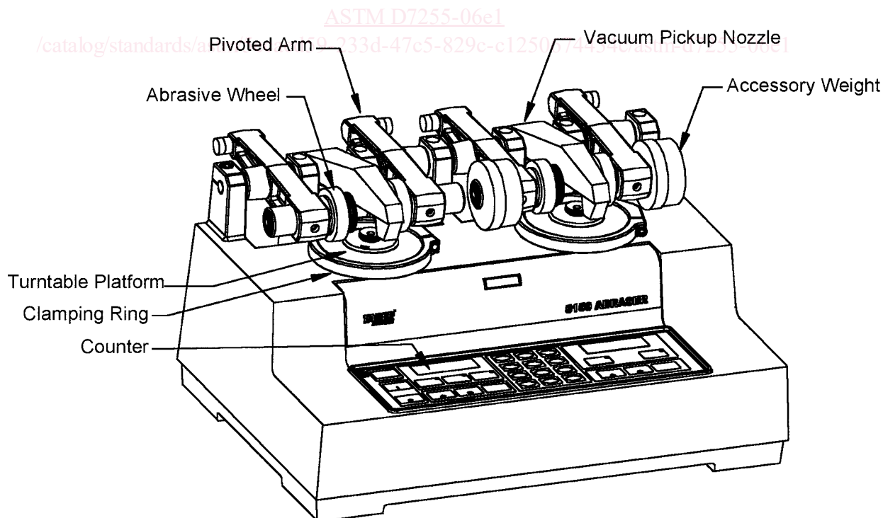
FIG. 1 Rotary Platform, Double-Head Tester
