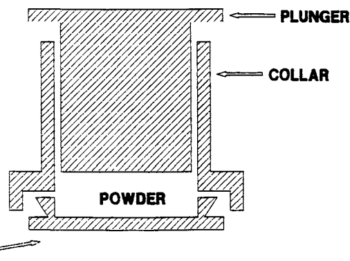
NOTE 1—The collar and receptacle should be securely held in place before pressing the powder.
