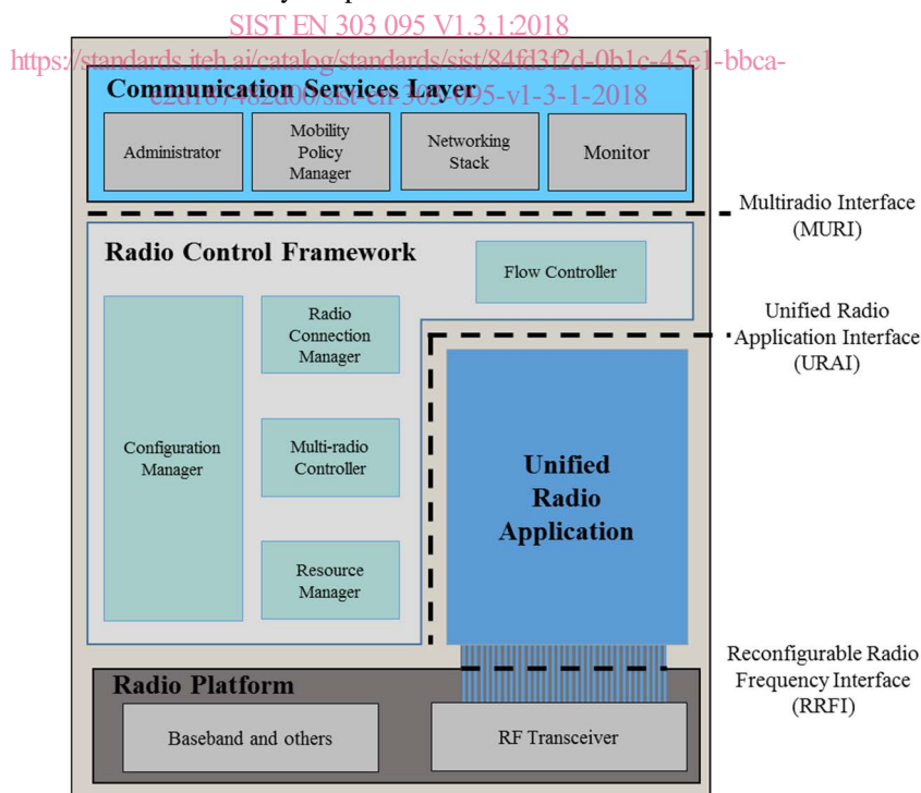
Figure 4.1: Reconfigurable mobile device architecture components for radio reconfiguration
