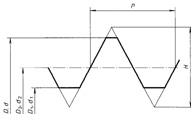
Figure 1 — Dimensions de base
