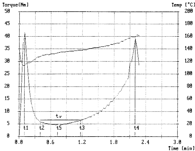
FIG. 1 Torque Rheometer Curve
