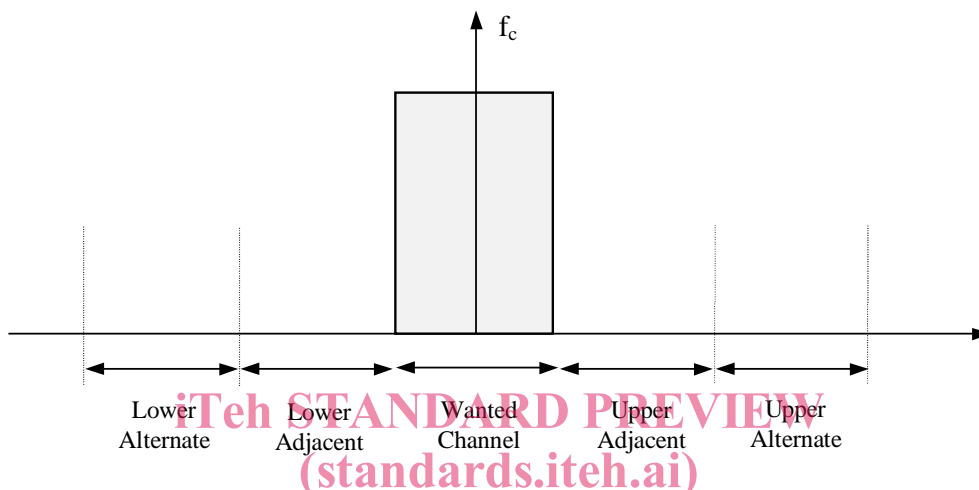
Figure 1: Adjacent and alternate channel definitions
