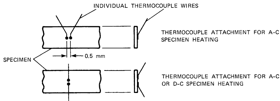
FIG. 6 Thermocouple Attachment
