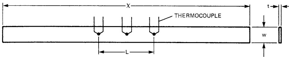
FIG. 4 Example of Emittance Sample in the Test Fixture
