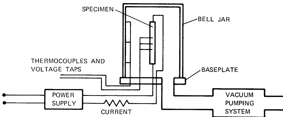
FIG. 1 System Arrangement
