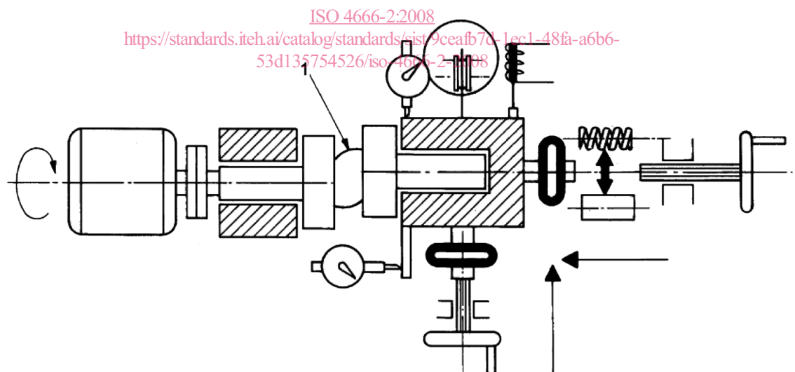
Figure 1 — Rotary flexometer before application of force
