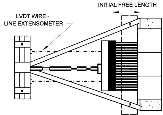
FIG. 2 Connection Test Apparatus (Plan View)
